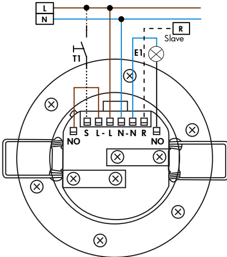
Wiring Diagram PD4-M-1C-FC
