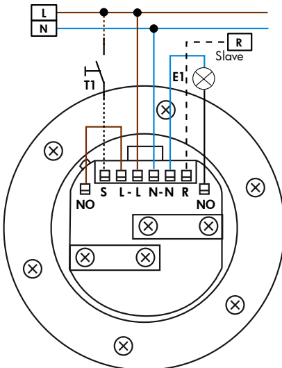
Wiring Diagram PD4-M-1C-FM
