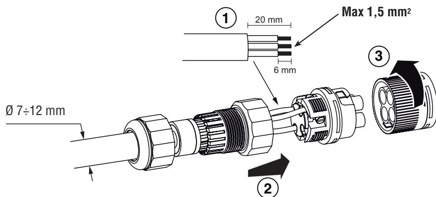
PLUG 4P
