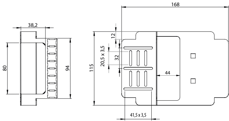
Metal termination box GW 38 339
