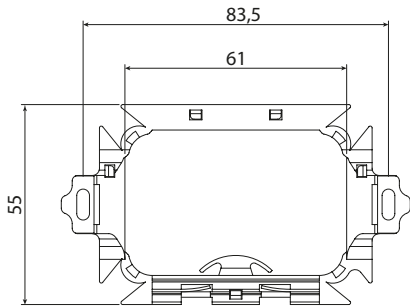
Splice holder cable spool GW 38 334
