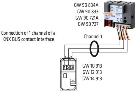
GW 10 913 GW 12 913 GW 14 913
