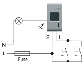
Multi-point light control and setting with NO push-buttons
