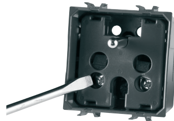
Terminal tightening screws
