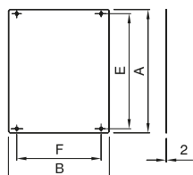
steel plates
