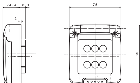
WATERTIGHT CAP WITH MEMBRANE - GW 27 401
