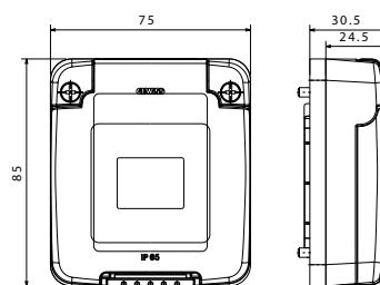
Watertight solid cap - GW 27 403
