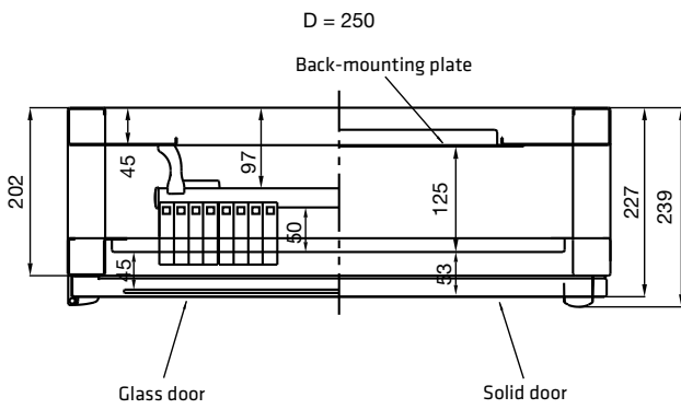
FLOOR-MOUNTING BOARDS
