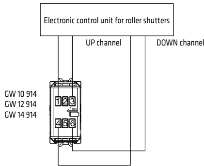
Connection to electronic control panel for moving roller shutters
