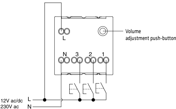
Connection diagram
