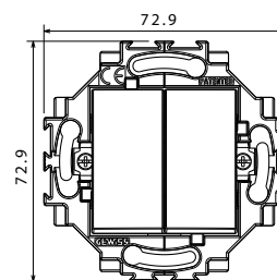
Double one-way switch (screwless) GW 35 051 W - GW 35 051 Y
