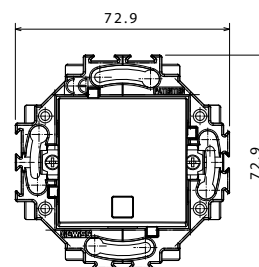
One-way switch with lens - backlit (screwless) GW 35 006 W - GW 35 006 Y
