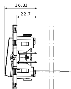
One-way switch with lens - backlit (screwless) GW 35 006 W - GW 35 006 Y
