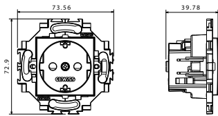
German std socket-outlet (screw) GW 35 207 W - GW 35 202 Y
