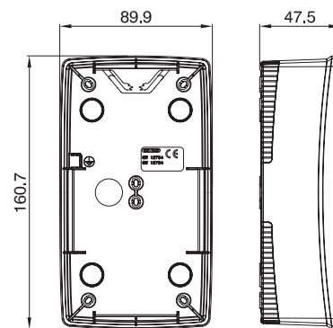
2+2 POSTI VERT. GW 16 754 - GW 16 784
