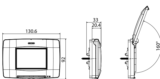
3 POSTI GW 16 703 TBN - GW 16 703 TNN - GW 16 703 VTN
