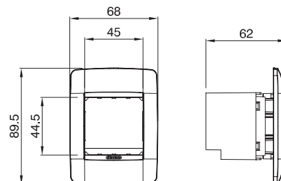
2 POSTI GW 16 712 TB - GW 16 712 TN - GW 16 712 VT
