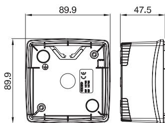
2 POSTI GW 16 752 - GW 16 782
