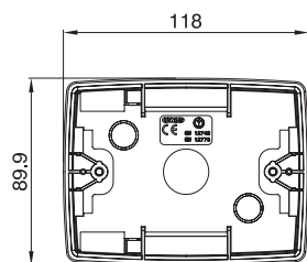
3 POSTI GW 16 743 - GW 16 773
