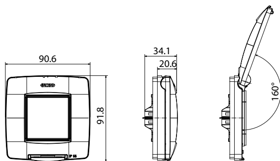
2 POSTI GW 16 702 TBN - GW 16 702 TNN - GW 16 702 VTN
