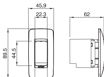
1 POSTO GW 16 711 TB - GW 16 711 TN - GW 16 711 VT
