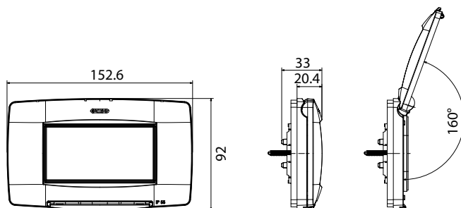
4 POSTI GW 16 704 TBN - GW 16 704 TNN - GW 16 704 VTN
