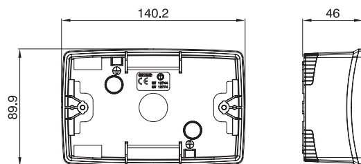
4 POSTI GW 16 744 - GW 16 774
