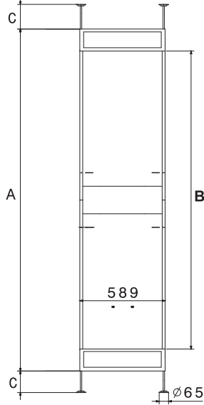
FLUSH-MOUNTING BACK-MOUNTING BOXES
